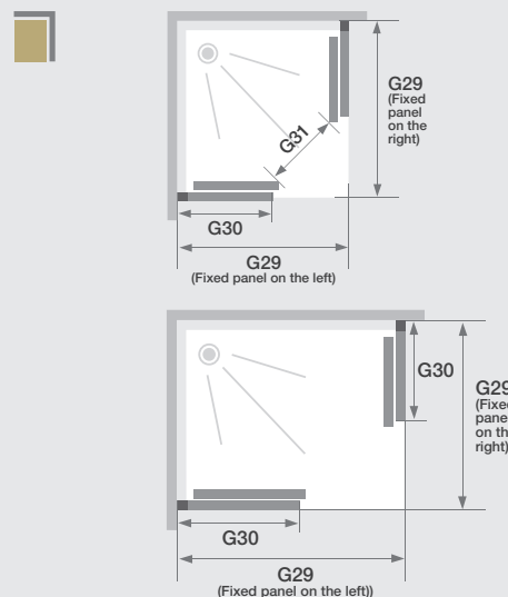
All measurements in mm
