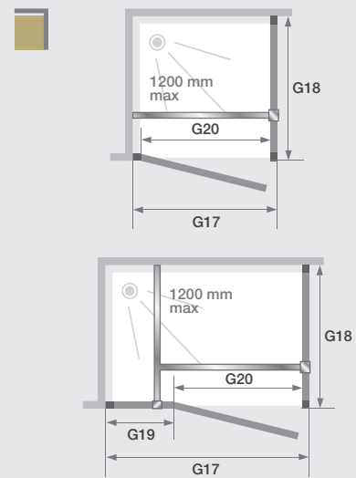
All measurements in mm
